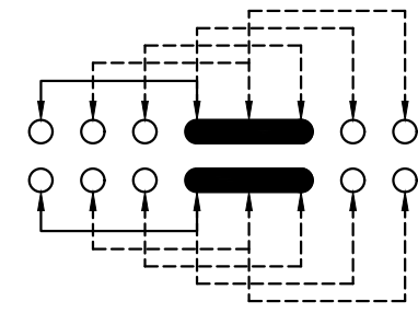
SCHEMATIC (SHORTING)
