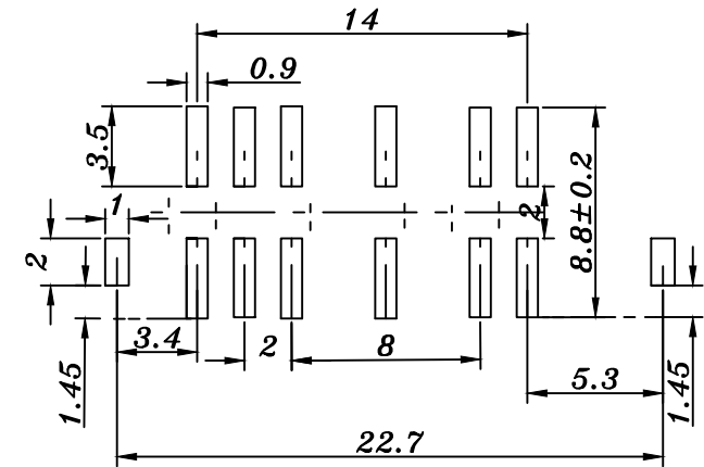
PCB LAYOUT
